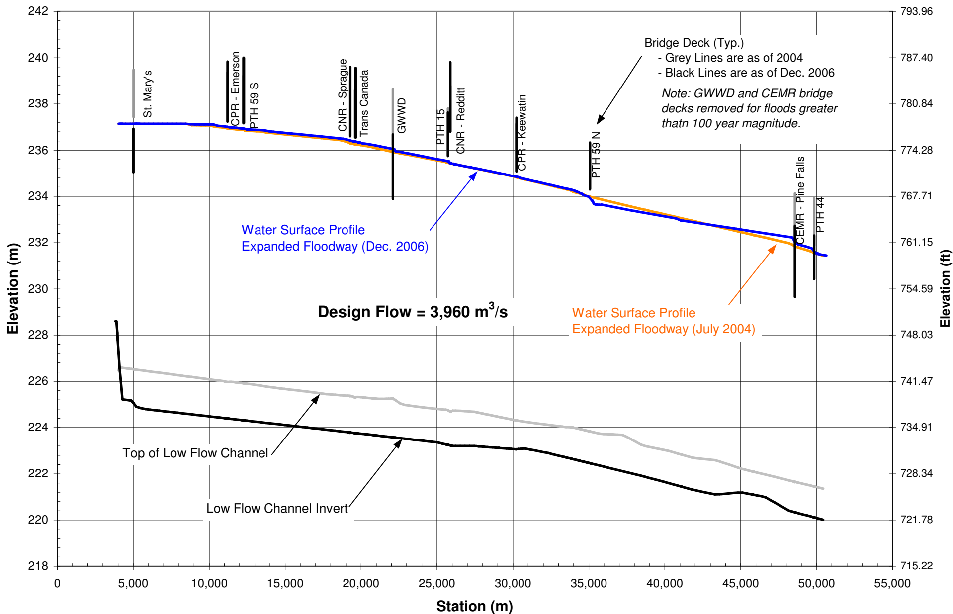
Figure 4.3-6 Water Surface Profiles for Expanded Floodway
