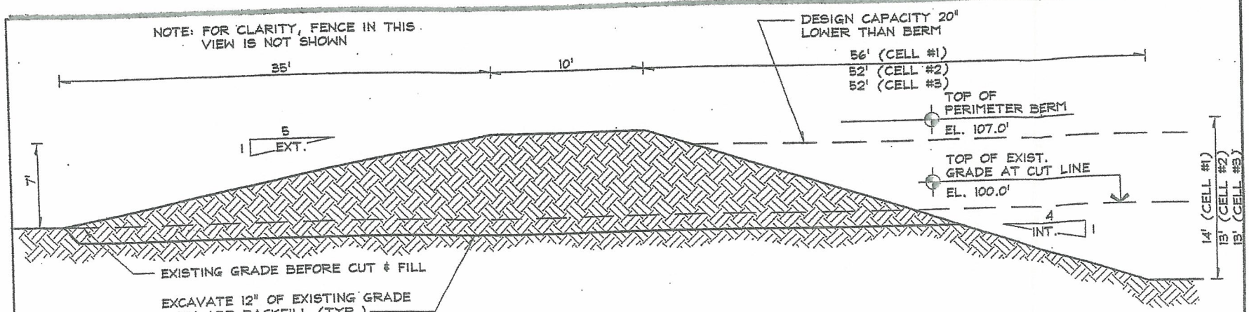
SECTION THRU PERIMETER BERM
