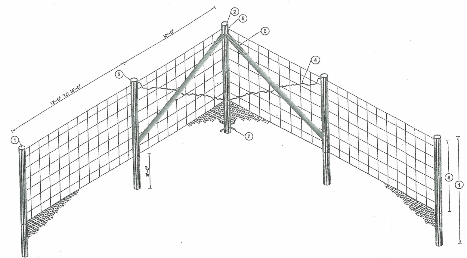
PAGE WIRE FENCE - ELEVATION VIEW
