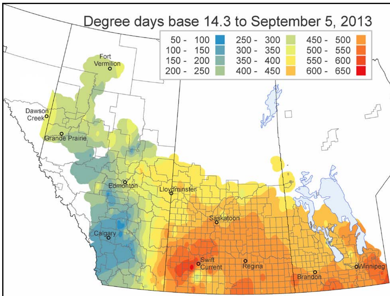
Figure 3 - Degree day accumulations, as of week 36, across the Prairie Provinces.
