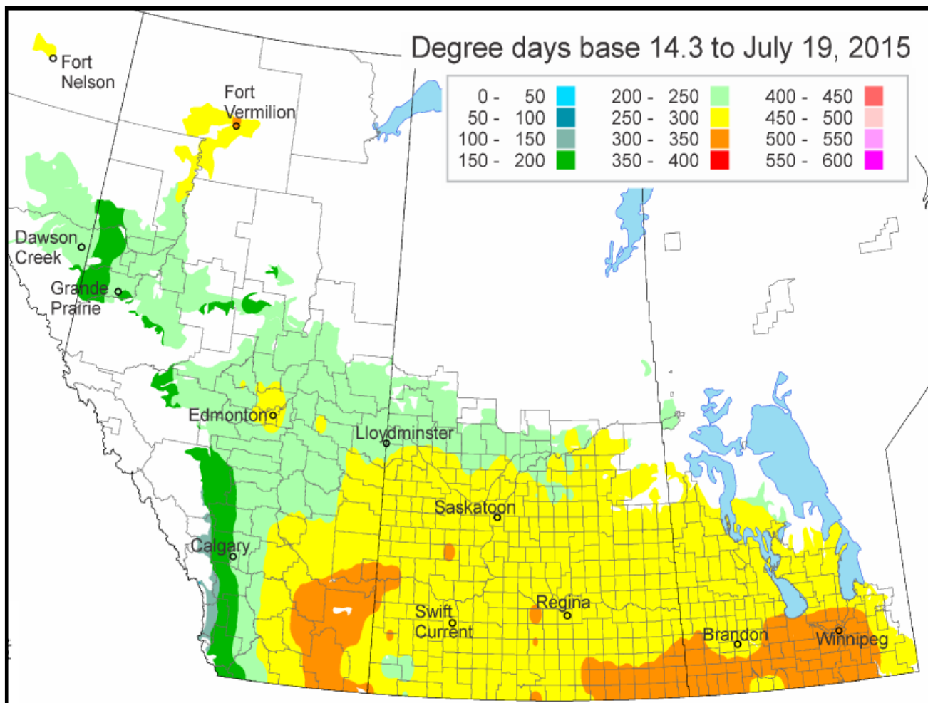
Figure 3 - Degree day accumulations, as of Week 28, across the Prairie Provinces.
