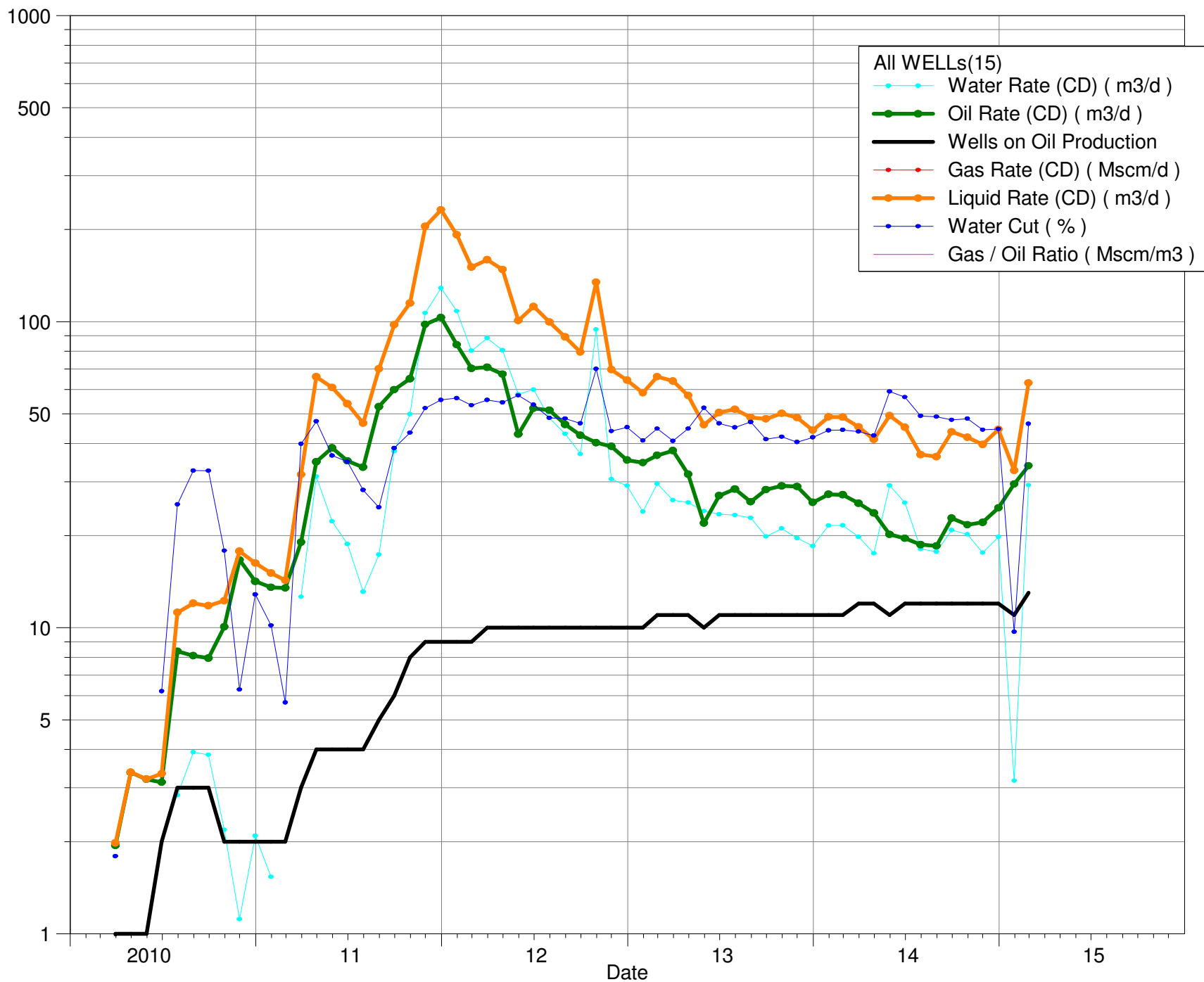
Proposed East Manson Unit No. 5 Historical Group Production Plot Figure 3
