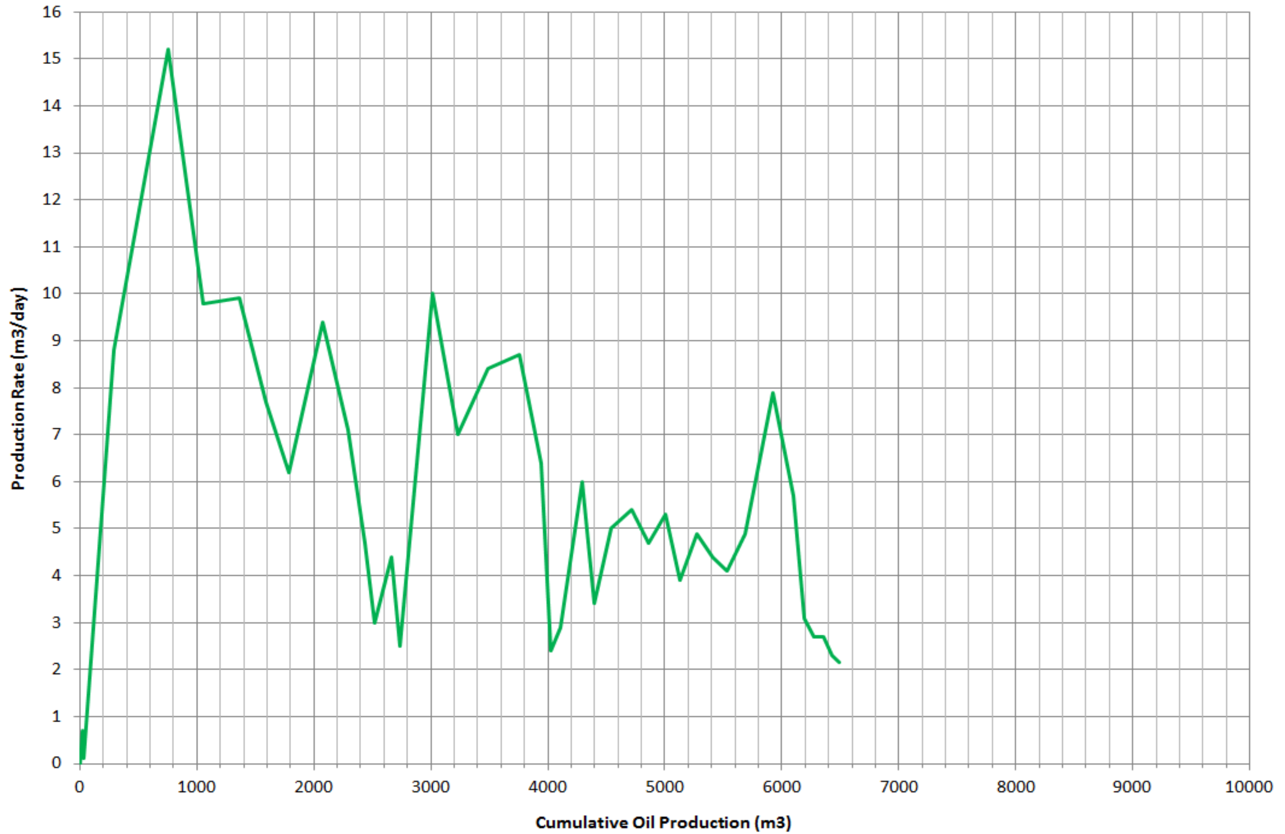
Appendix C, Figure 3: S ½ & NW ¼ SEC 28-13-29W1 Production Rate vs Cumulative Production
