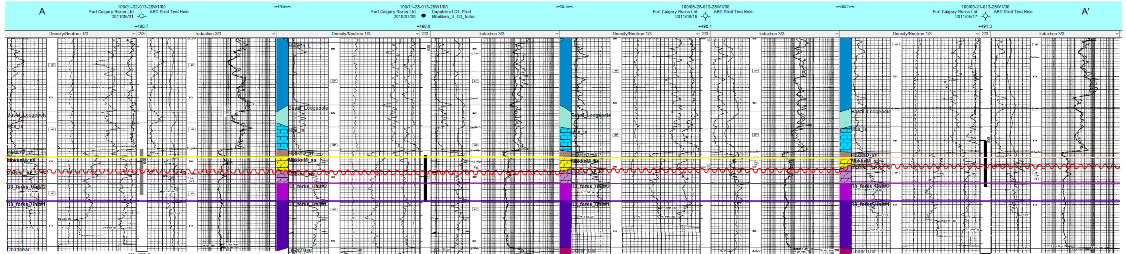
Appendix B, Figure 11: Stratigraphic Cross Section A-A' (Northwest to Southeast) across EMU No.6
