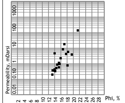
Core: Porosity Statistics [mts] Samples 19, 664.9 - 670.4
