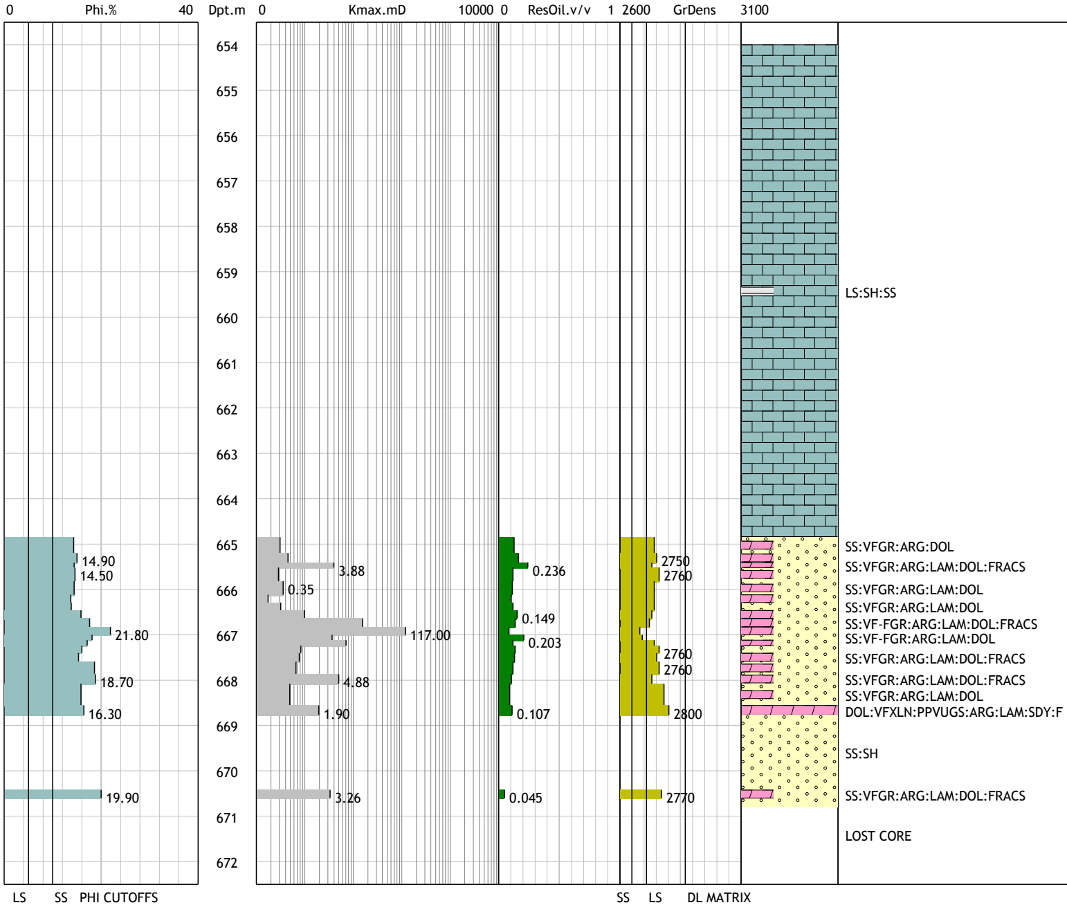
Core: Perm.Kmax vs Phi Samples 19, 664.9 - 670.4
