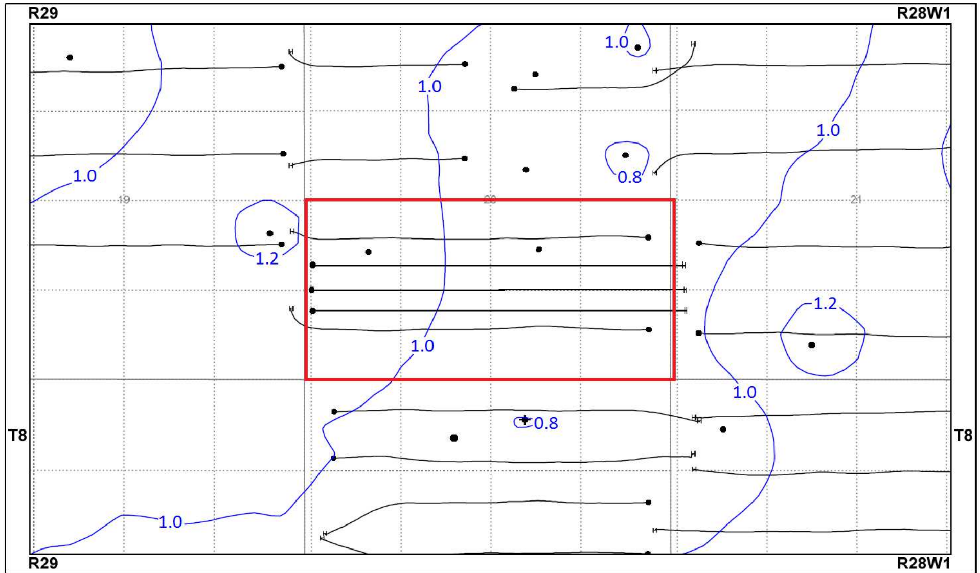
Lodgepole Dolomite Phi-h (0.2m CI) Map Showing Vertical Wells and Lodgepole Producing Horizontal Wells
