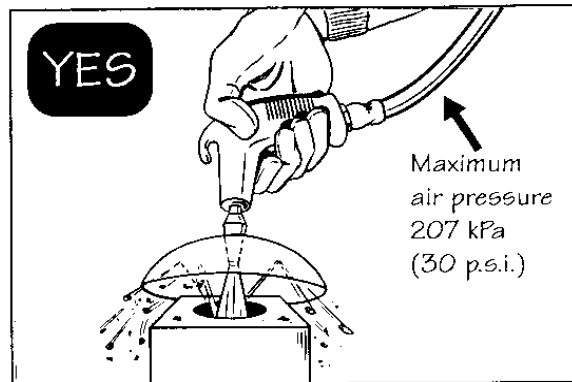
Blowing WITH chip guard
