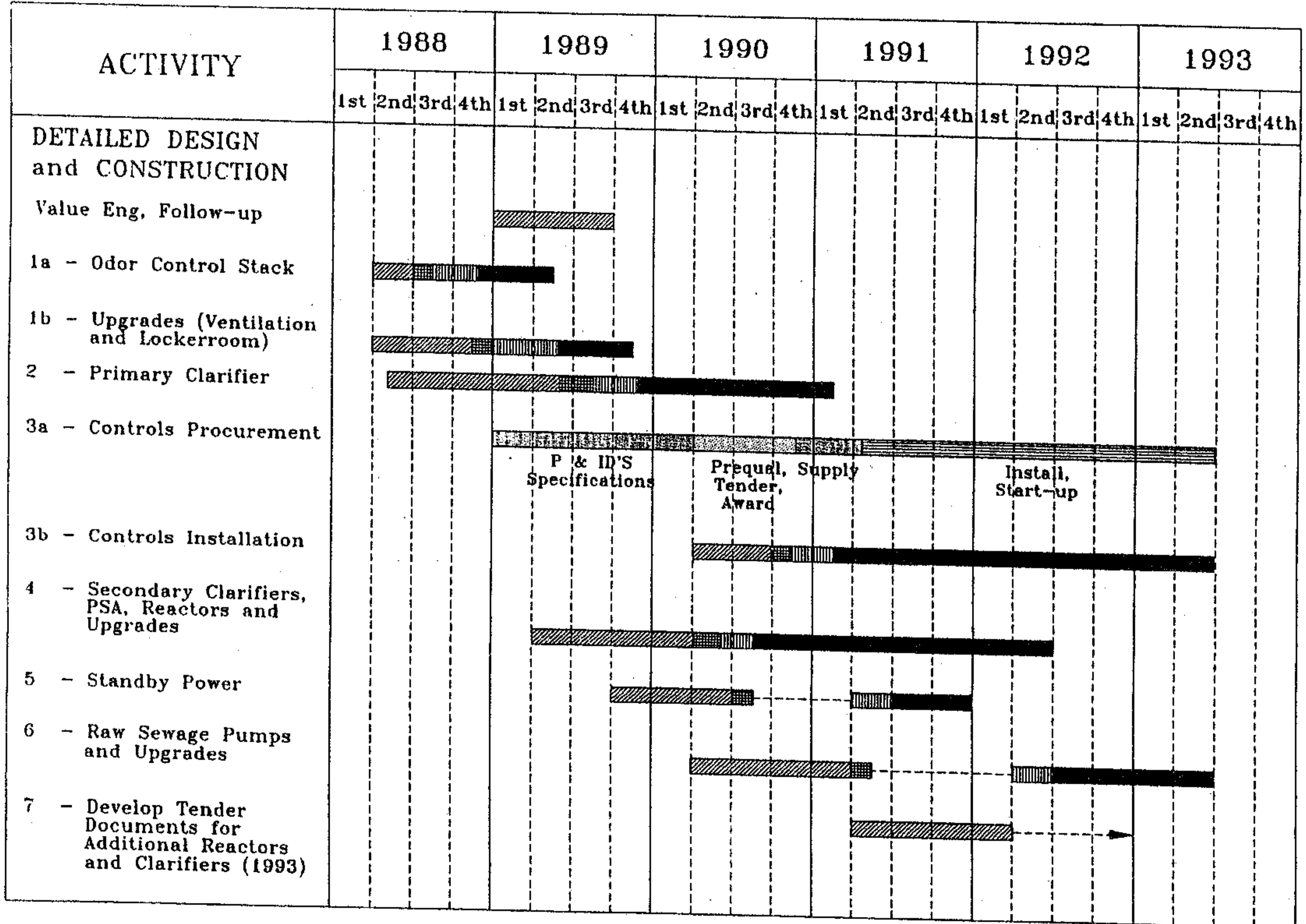
SEWPCC EXPANSION Stage 1 Schedule Overview Figure 17-1
