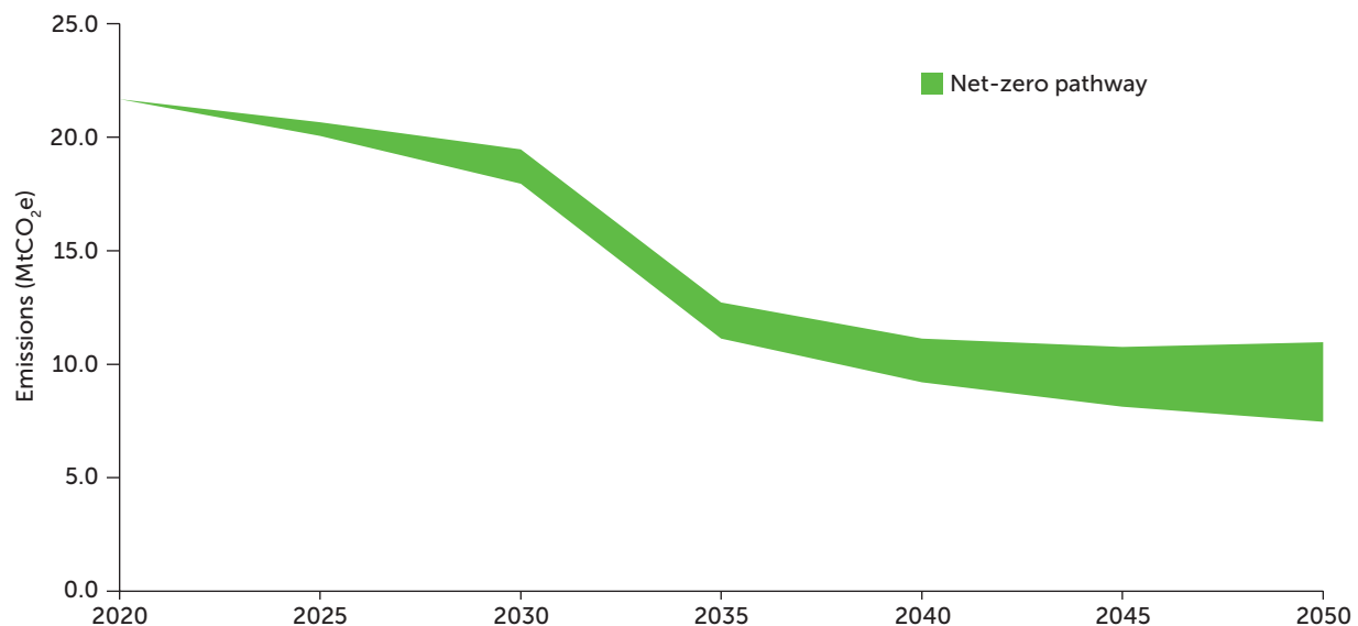
Figure 6: Manitoba's net-zero pathway
