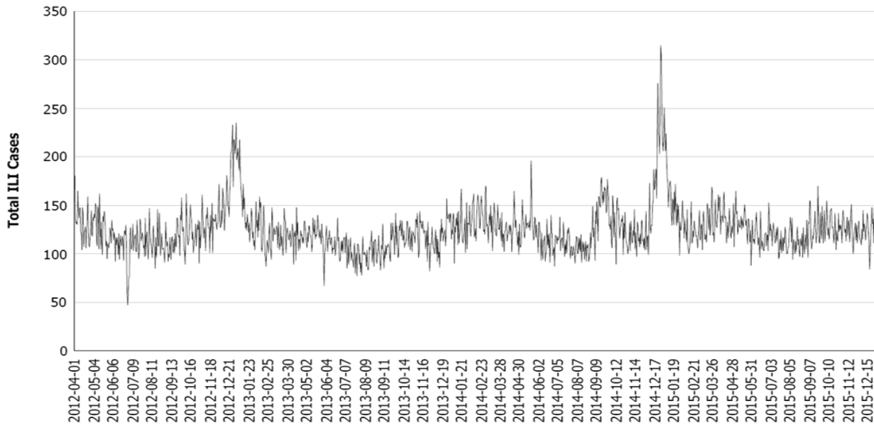
Figure 5 ILI cases in Emergency Department at WRHA, Manitoba
