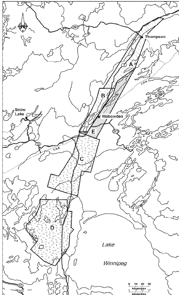
Figure GS-4-1: Compilation progress in the Thompson Nickel Belt.
