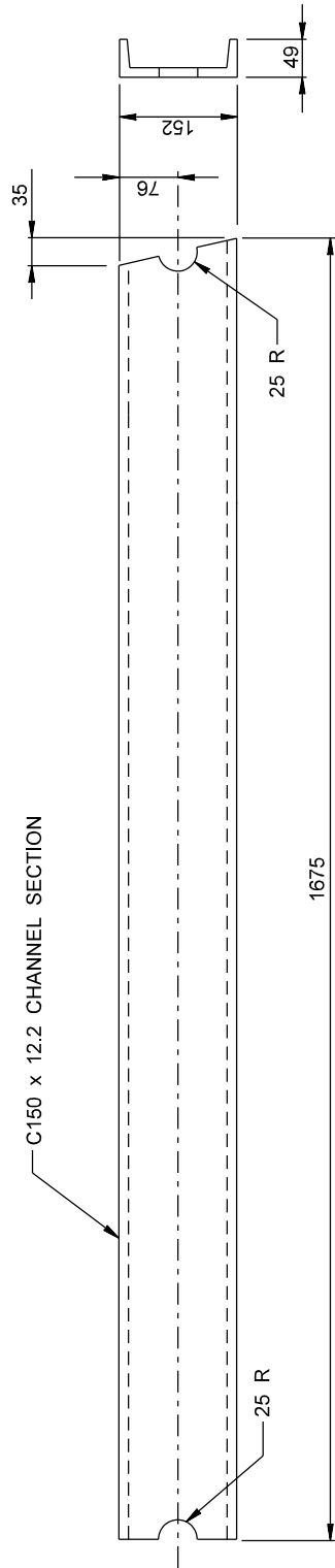
YOKE DETAILS 1:10 (2 REQUIRED)
