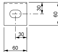
SECTION C-C 1:5
