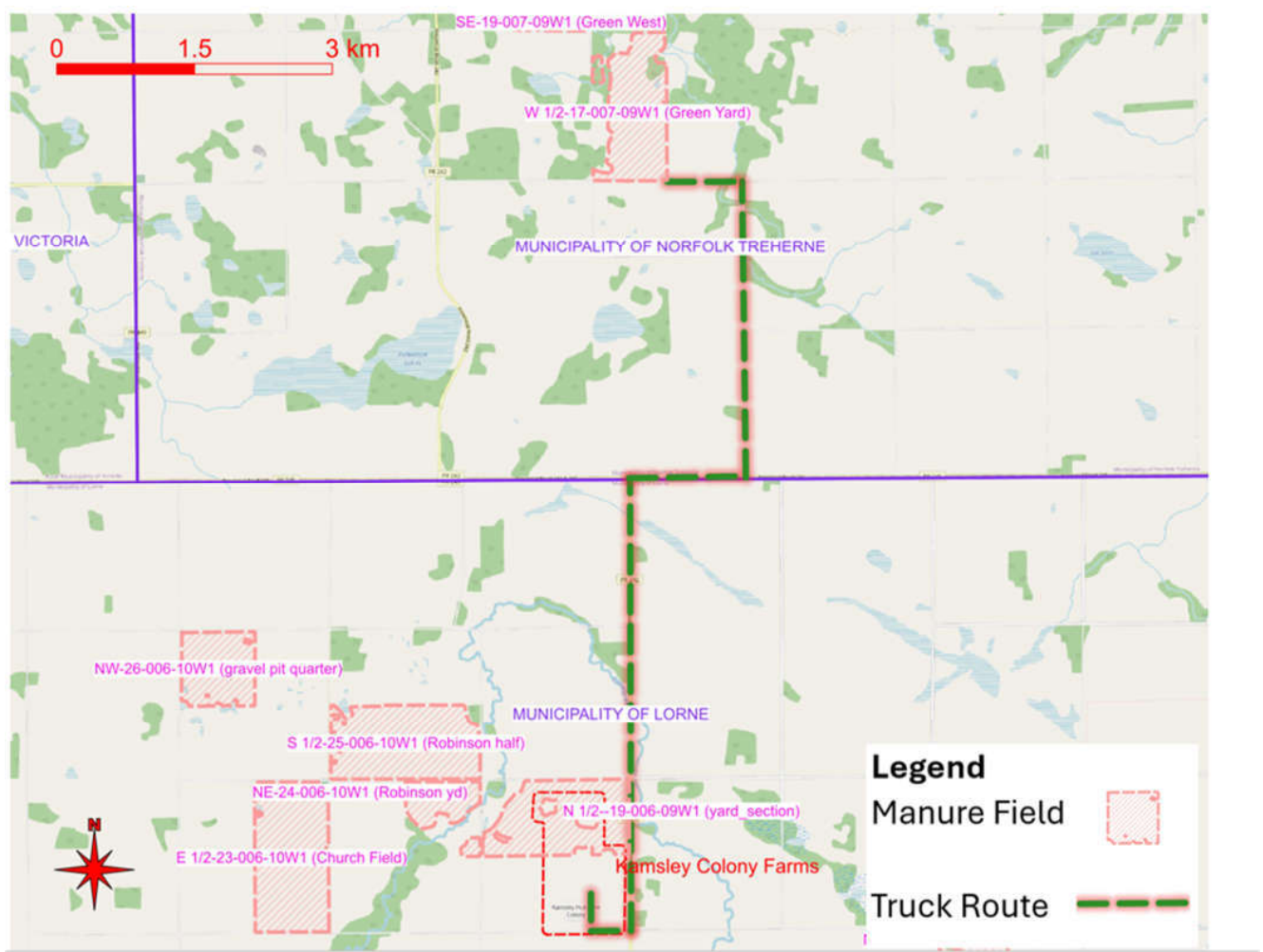
FIGURE 7: PRIMARY MANURE HAULING ROUTE
