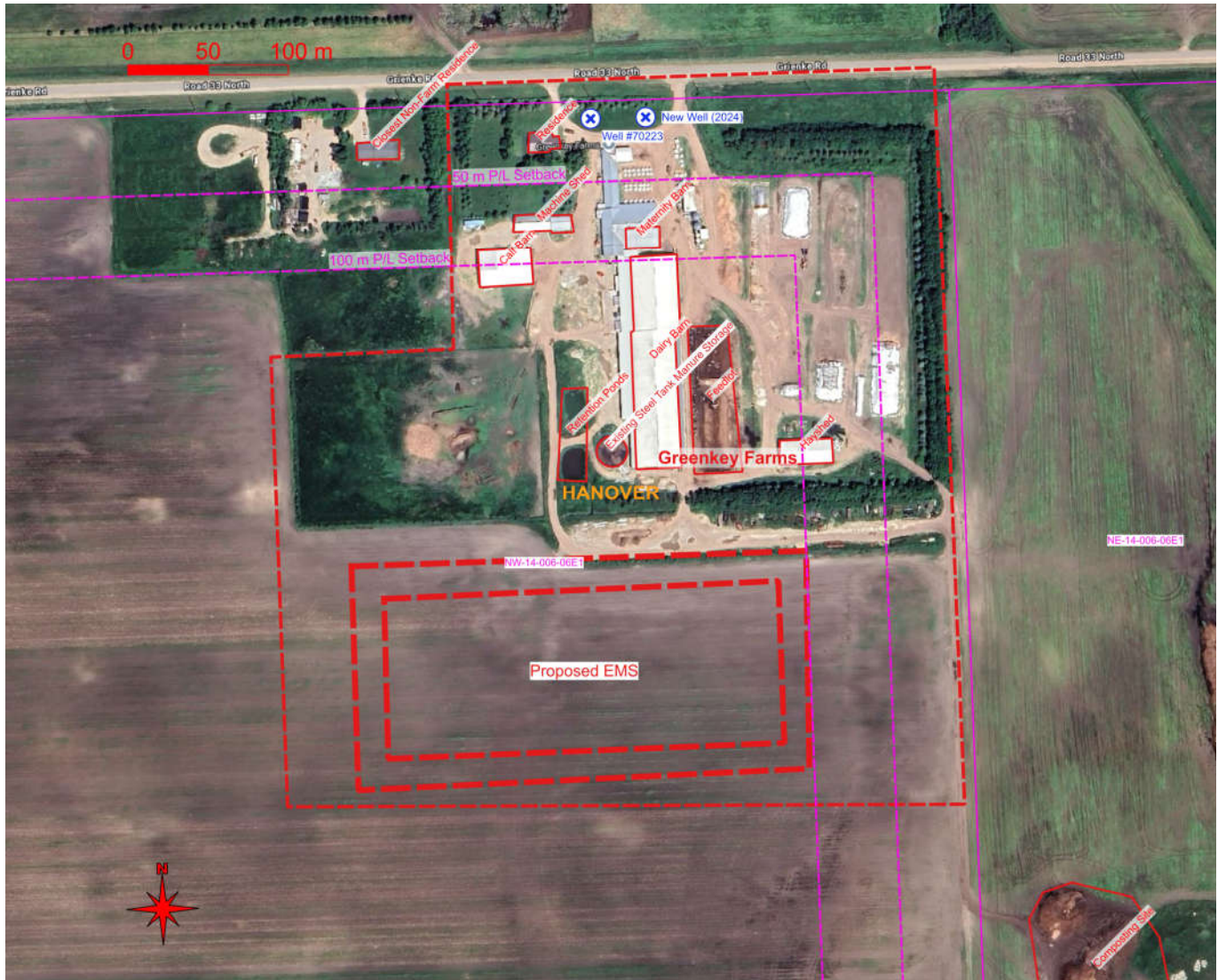
Figure 2: Greenkey Farms (NW-14-006-06EPM) Site Plan
