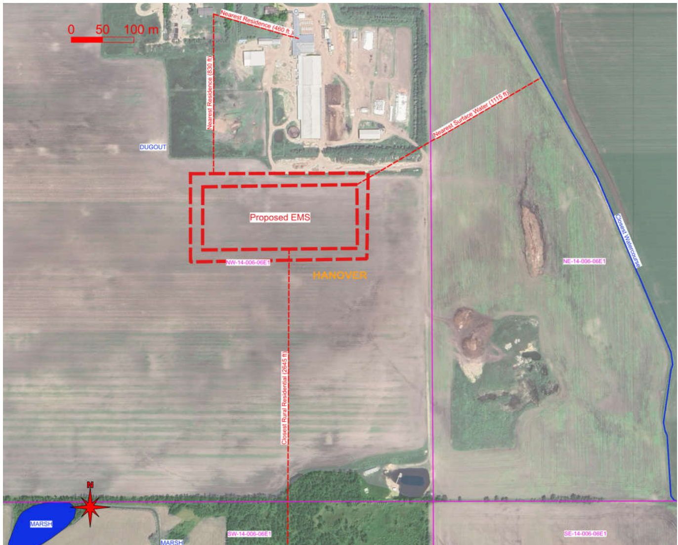
Figure 6: Separation Distances.
