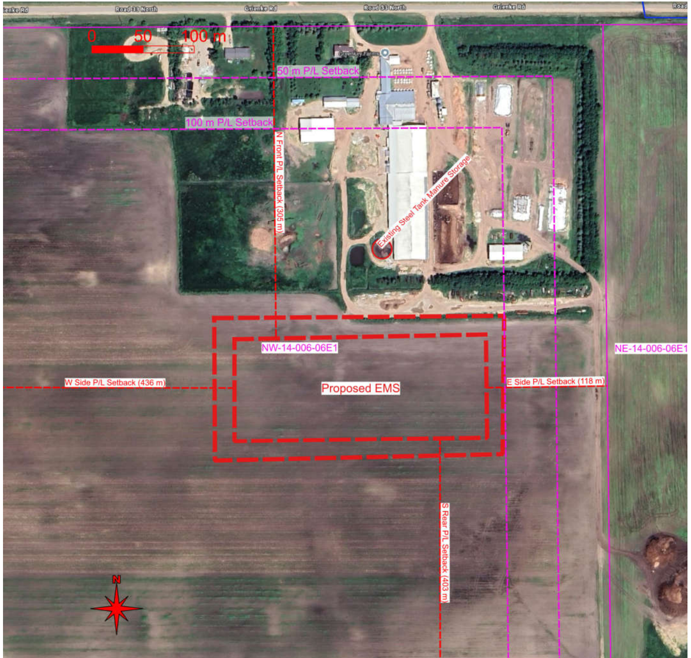
Figure 4: Setback Distances for Proposed New Manure Storage
