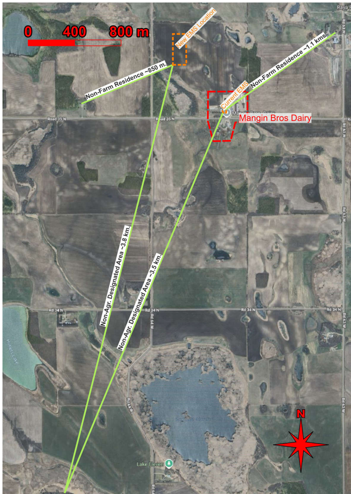
Figure 5: Separation Distances (Manure Storages).
