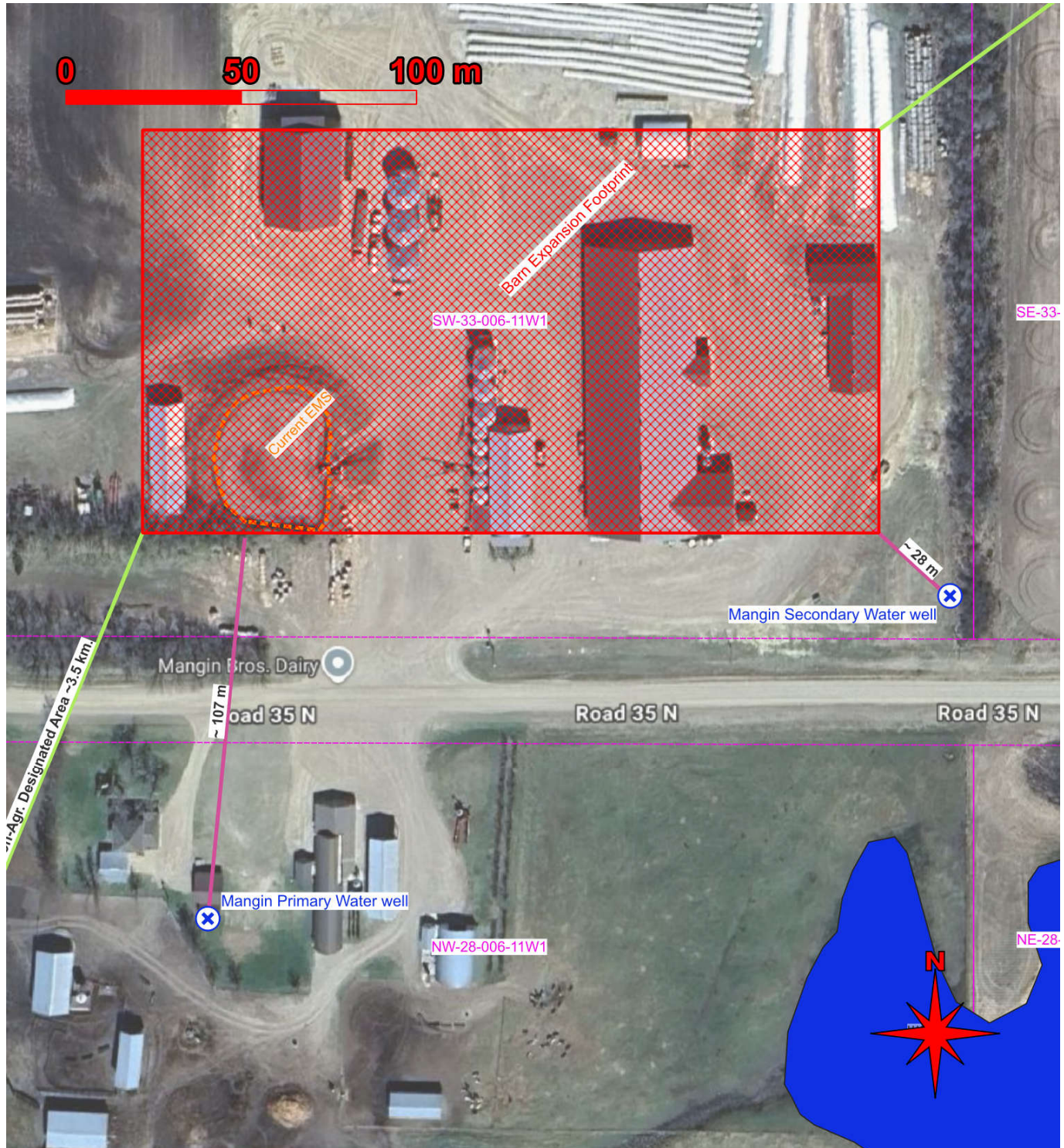
Figure 7: Separation Distances (Wells)
