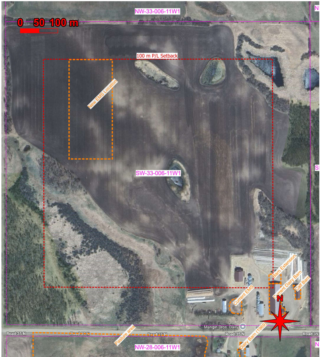
Figure 4: Property Line Setback Distances for Proposed New Manure Storage
