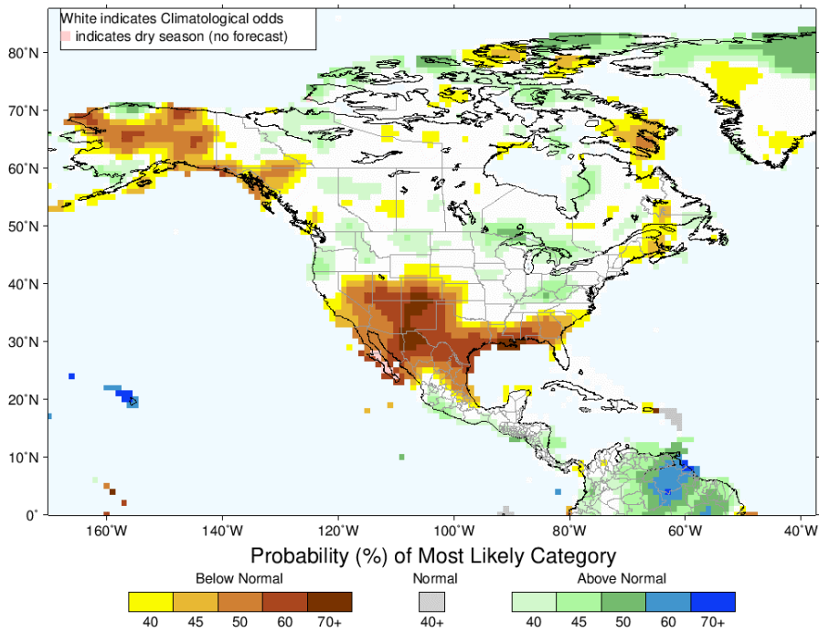
Figure 10 – IRI Multi-Model Probability Forecast for Precipitation for March–April–May 2022, issued February 2022.
