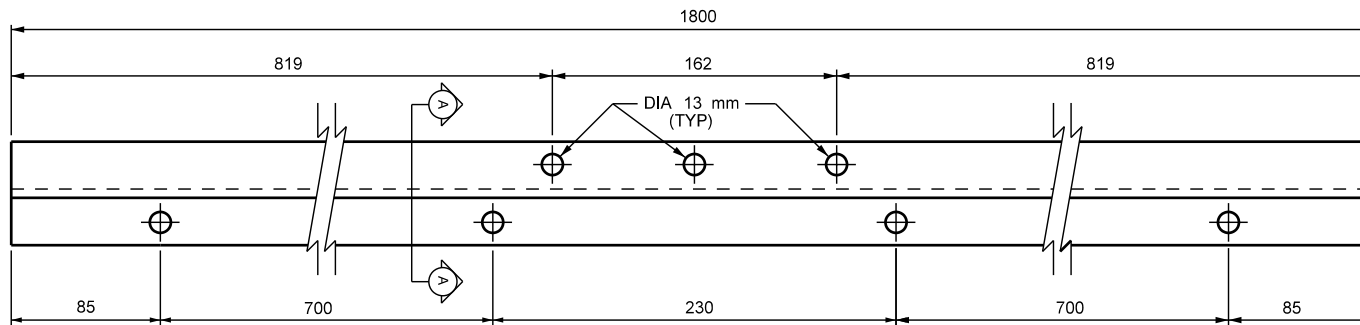
PLAN VIEW
