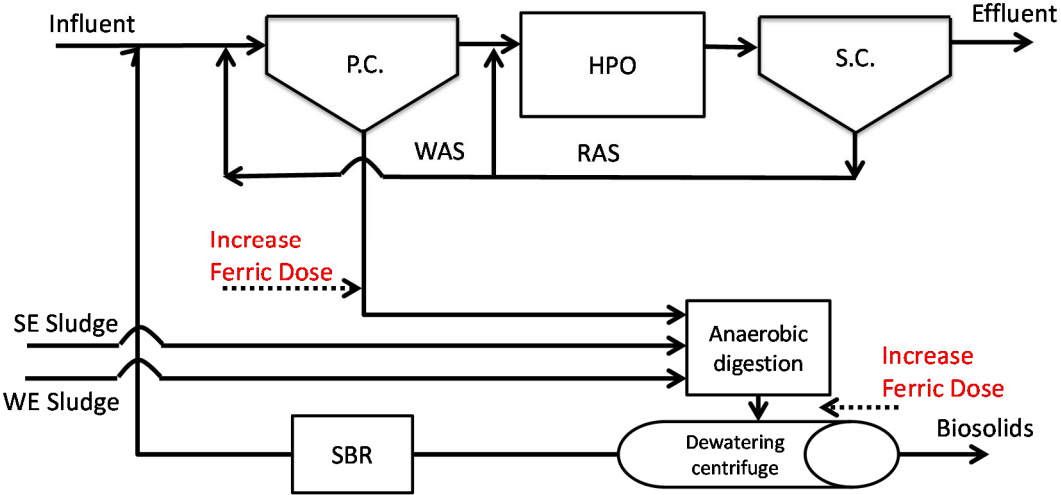
Figure 2: Increase Sidestream Chemical Phosphorus Removal
