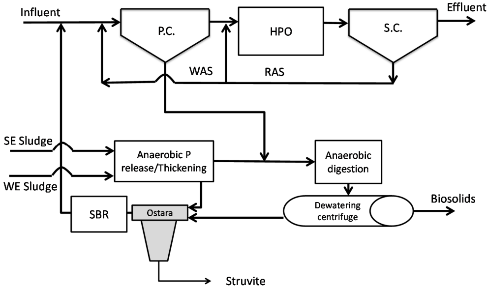
Figure 3: Sidestream Struvite Crystallization
