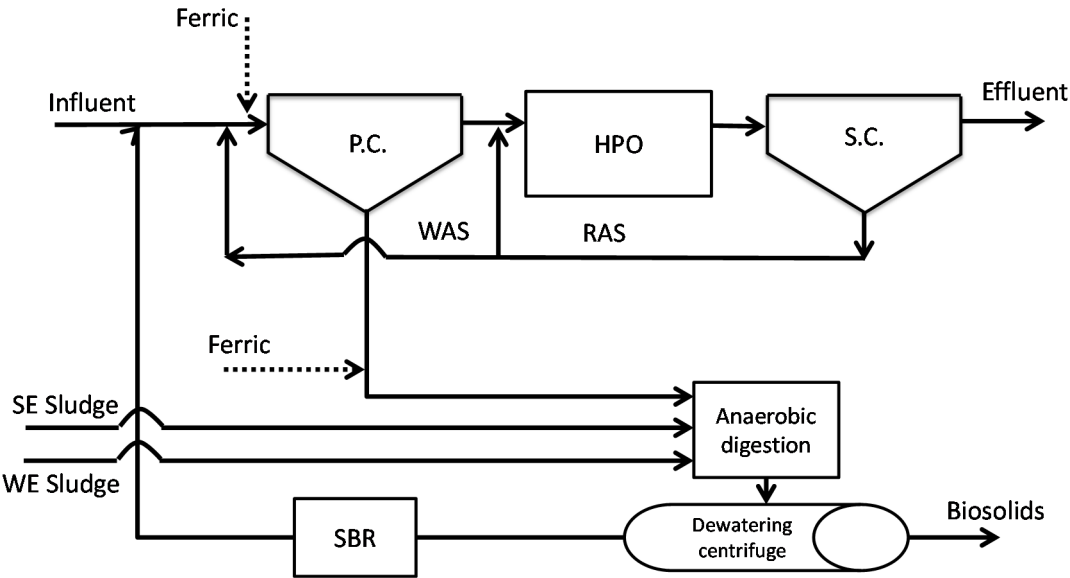
Figure 5: Chemically Enhanced Primary Treatment at the NEWPCC
