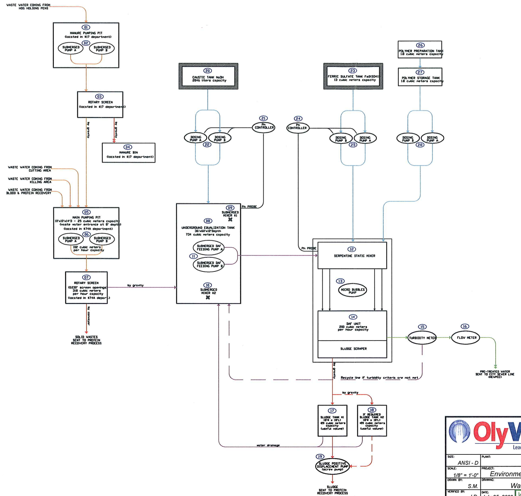
SCHEMATIC DIAGRAM
