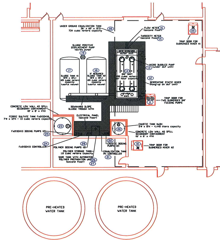
WASTE WATER ROOM LAYOUT
