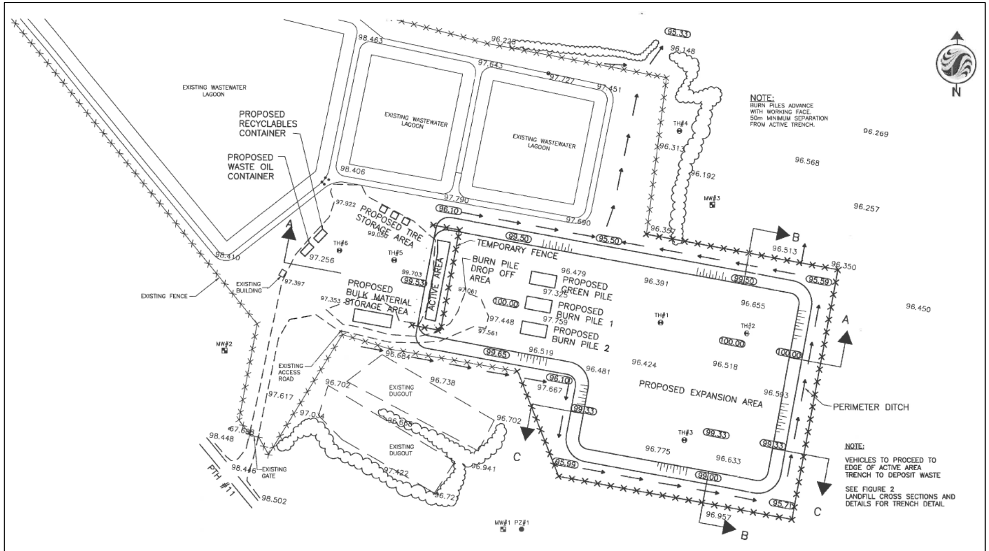
Figure 1 Facility Layout
