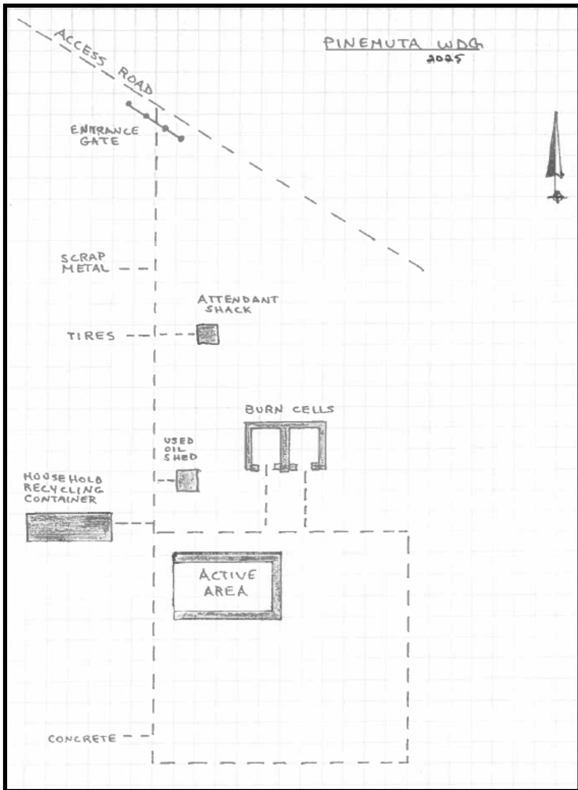
Figure 1 Facility Layout
