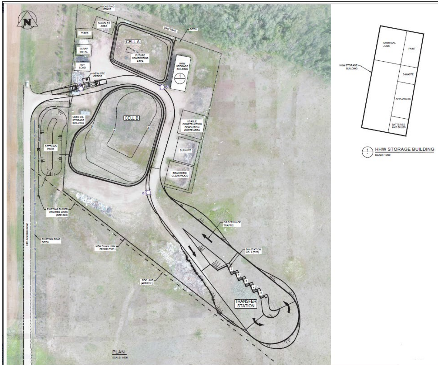
Figure 1: Clanwilliam-Erickson Waste Transfer Station Facility Layout
