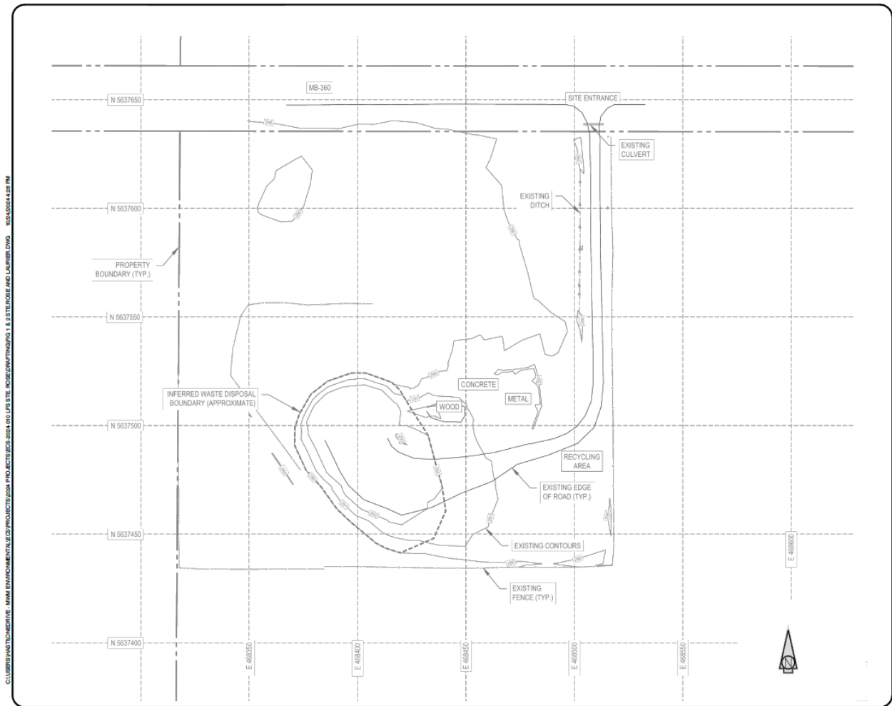
Figure 1 Facility Layout
