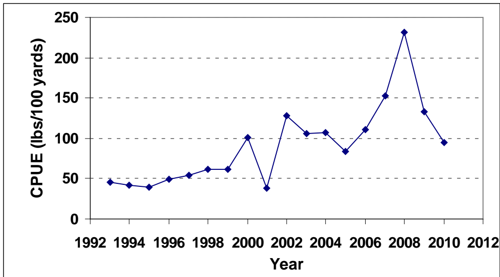
Figure 6: Catch-per-unit-effort of all walleye caught during annual monitoring in June, 1993 to 2010.
