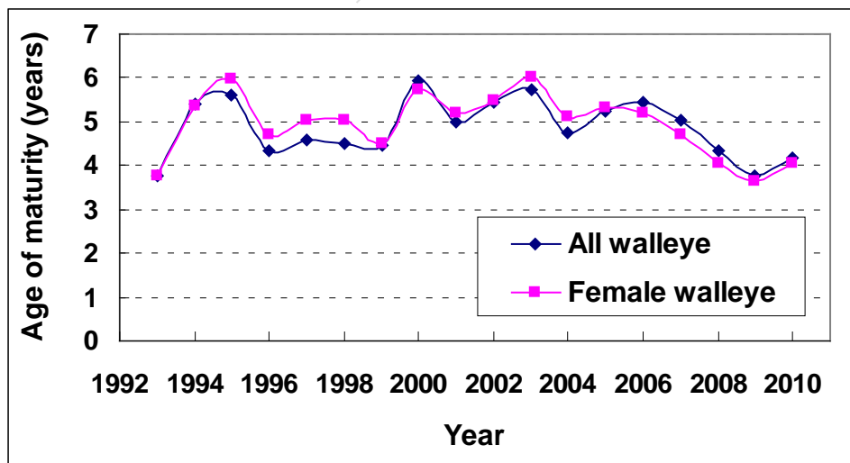
Figure 8: Age of maturity of walleye (sexes combined and females only) from annual monitoring in Dauphin Lake, 1993 to 2010.
