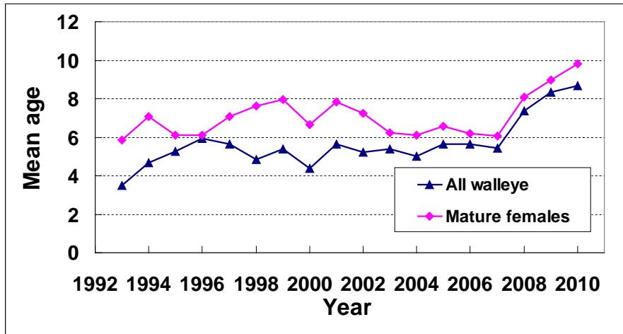
Figure 5: Mean age of walleye (sexes combined and mature females only) from 1993 to 2010.
