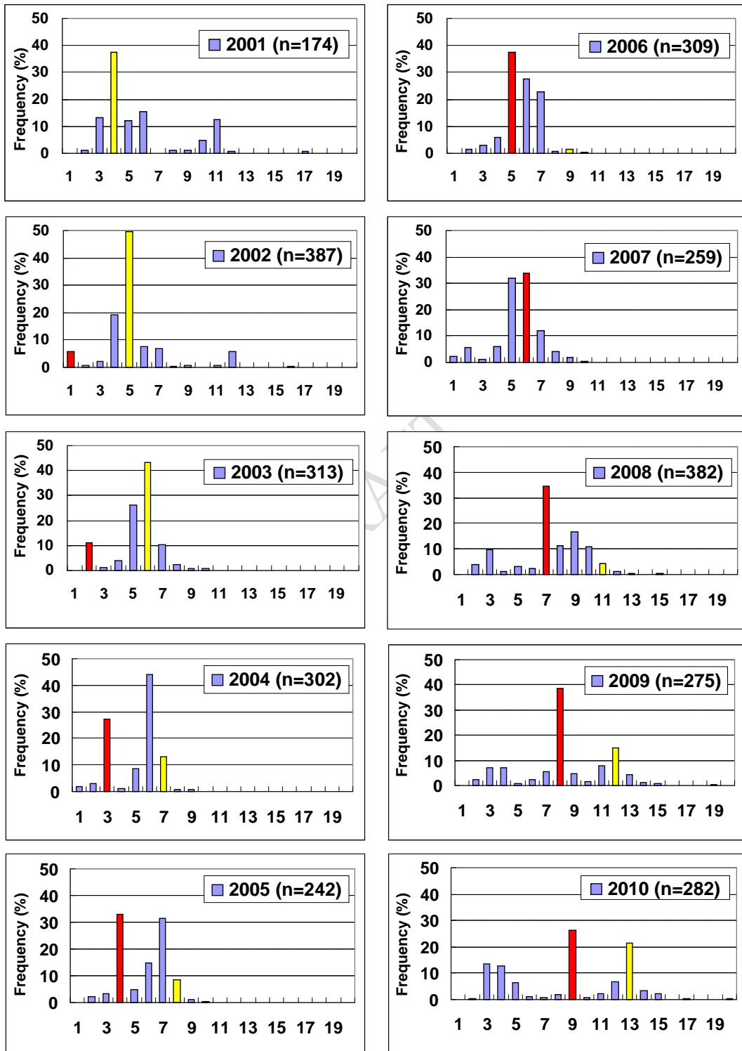
Figure 1: Age composition of walleye from index gill net surveys from 2001 to 2010.
