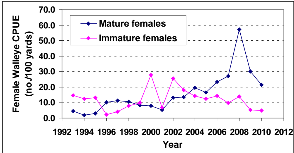
Figure 7: Catch-per-unit-effort of mature and immature female walleye caught during annual monitoring in June, 1993 to 2010.
