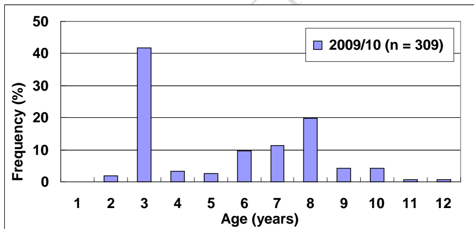
Figure 2: Age composition of walleye sampled from the 2009/10 winter commercial fishery
